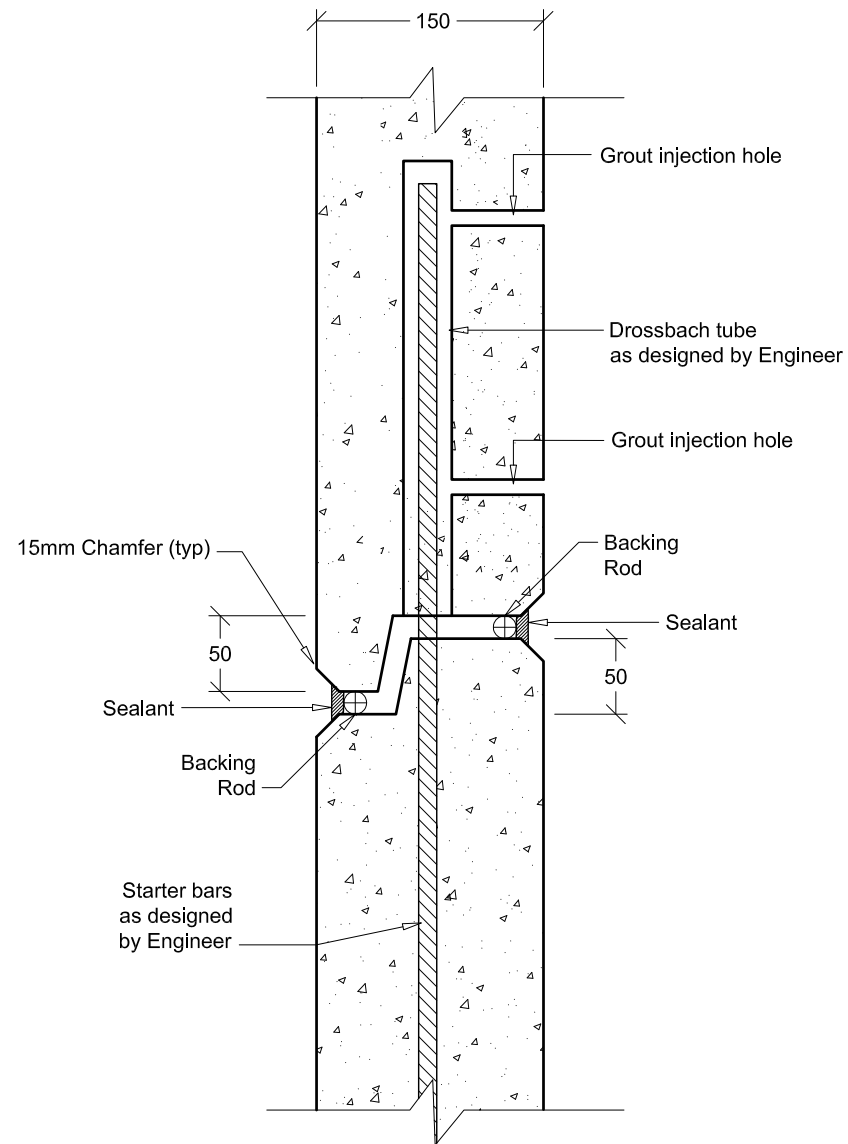
B20 TYPICAL HORIZONTAL JOINT DETAIL Scale 1:5
