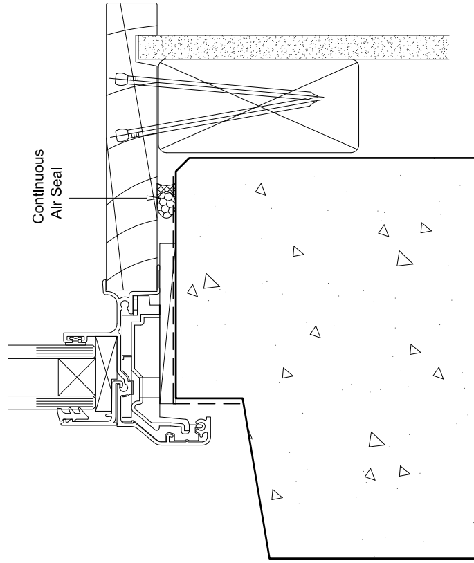
Sill Detail
