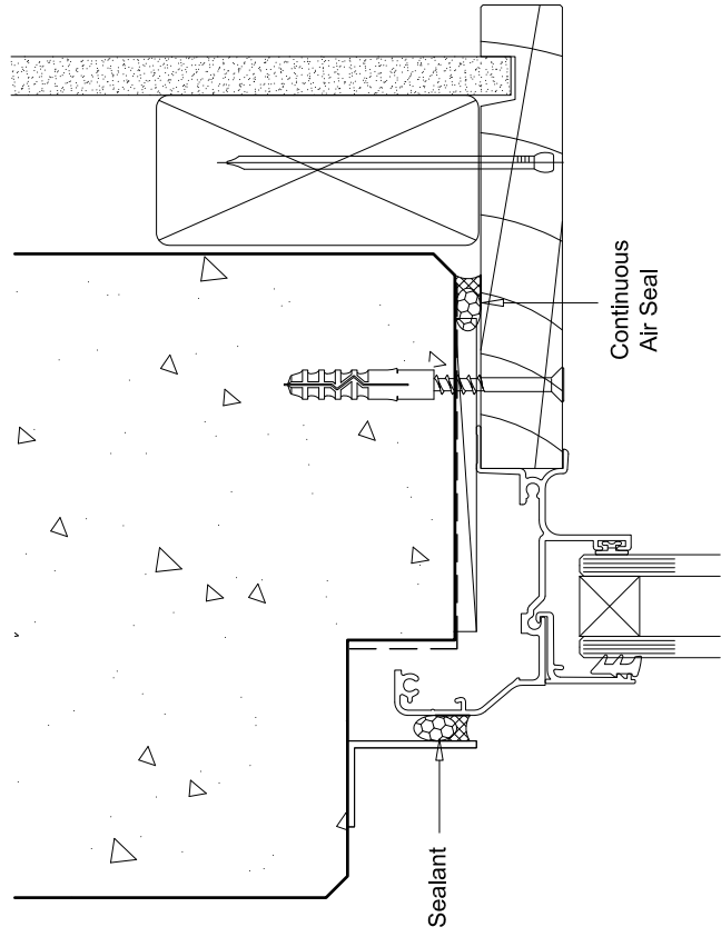
Head Detail
