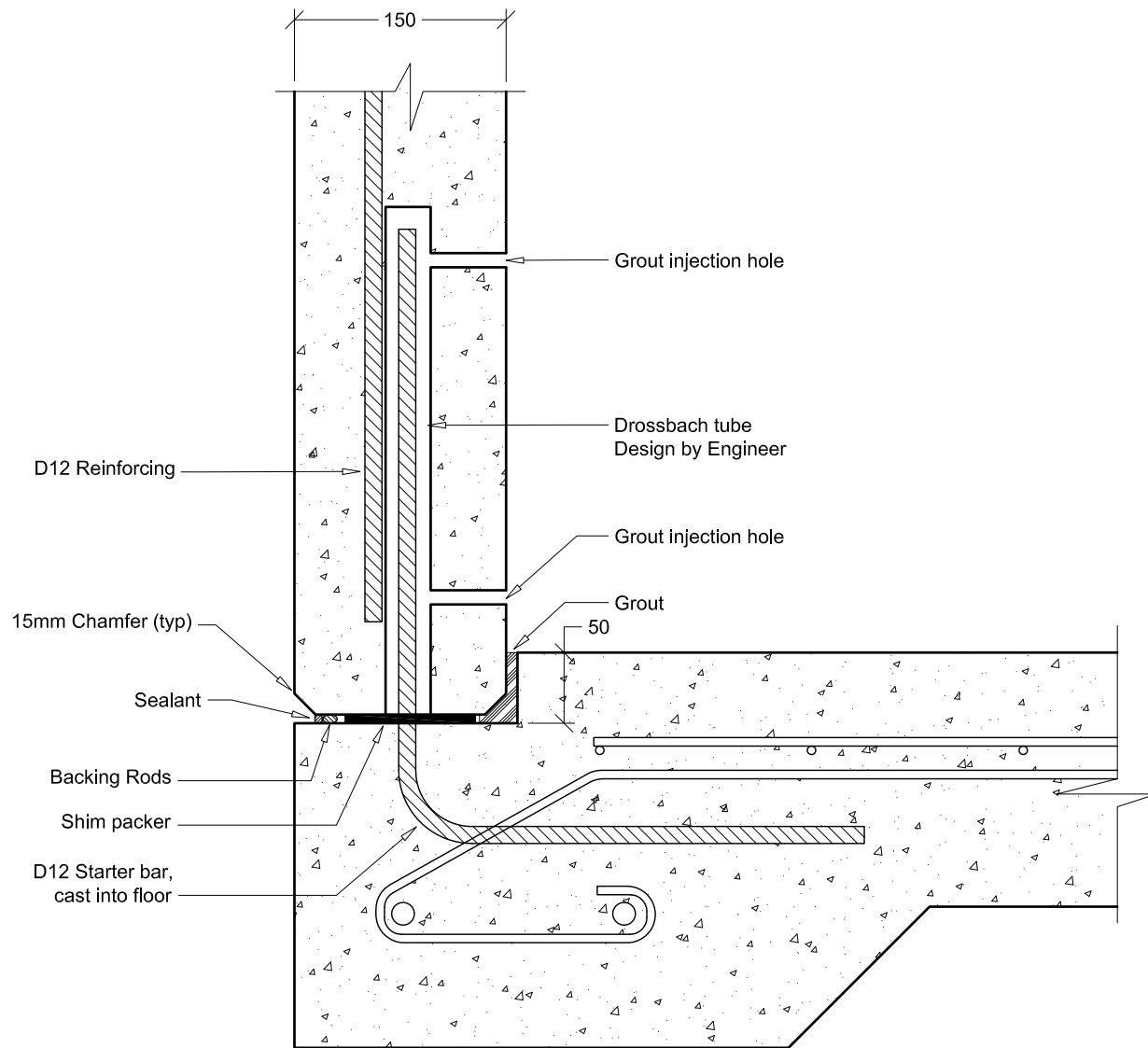
B3(2) TYPICAL PANEL JOINT DETAIL - PANEL / FLOOR SLAB CONNECTION (OPTION 2)
