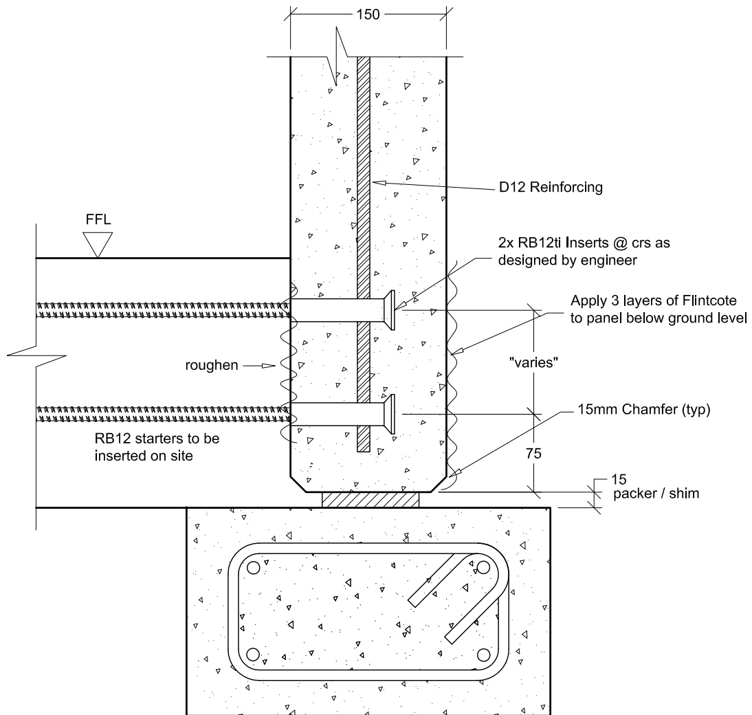
B3(3) TYPICAL PANEL JOINT DETAIL - PANEL / FLOOR SLAB CONNECTION (OPTION 3) Scale 1:5
